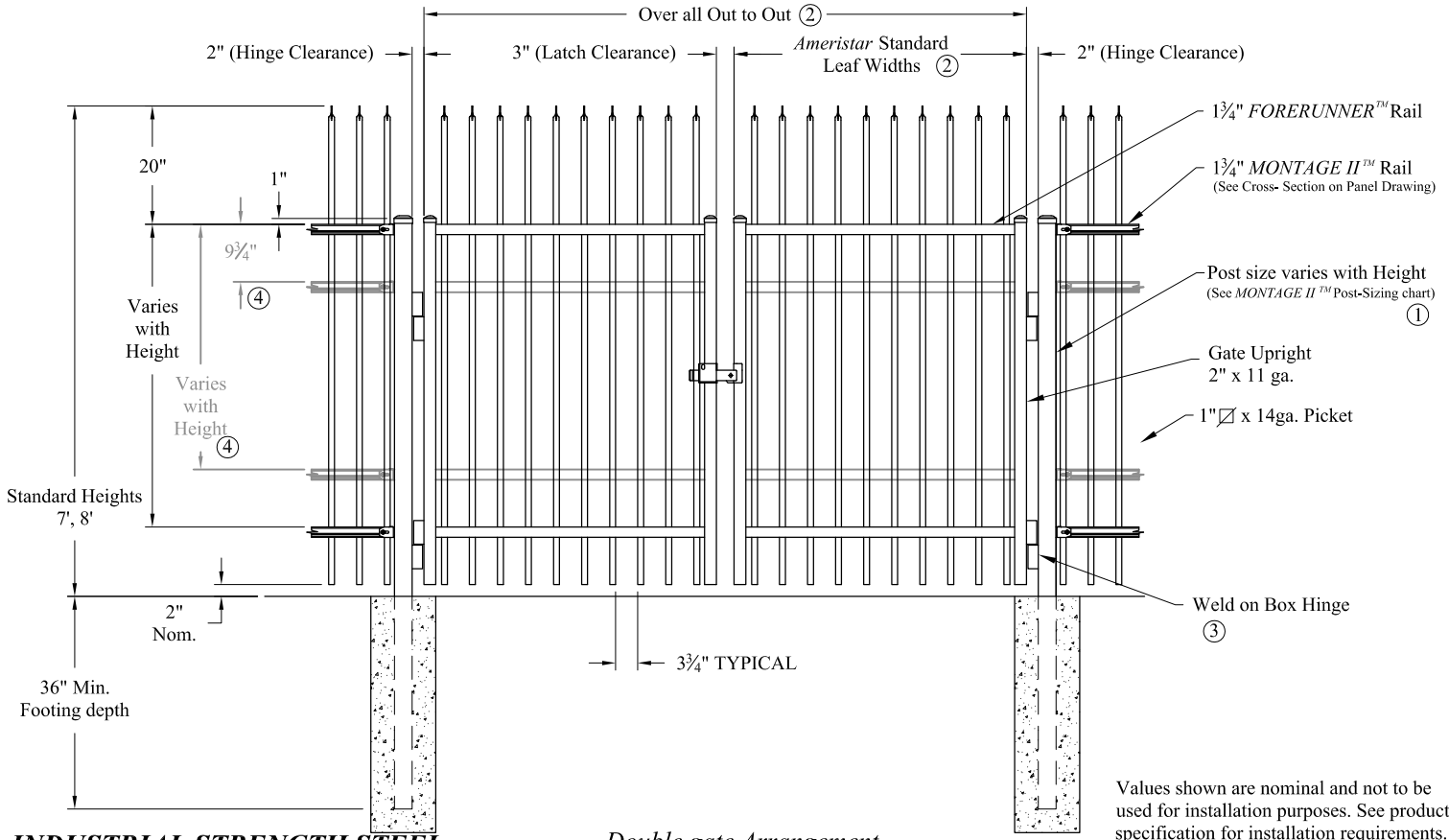
Double gate Arrangement
