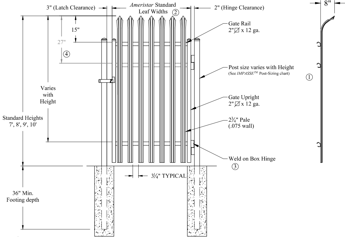
Single gate Arrangement
